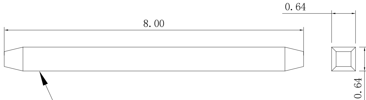
插针-单针直脚无塑- (0.64 方针 L=8.0mm 镀全金0.8U) -1P-0.64*8.0-RoHS
